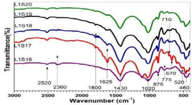
Figure (2). FTIR spectra of soil samples.
